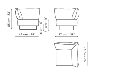
Corner 97x97 Width: 97cm Depth: 97cm Height: 85cm
