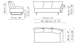
End section sofa 190-200 Width: 190-200cm Depth: 97cm Height: 85cm
