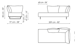
Meridiana Width: 97cm Depth: 209cm Height: 85cm
