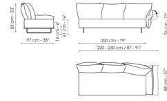
End section sofa 220-230 Width: 220-230cm Depth: 97cm Height: 85cm
