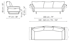
Sofa 240-260 Width: 240-260cm Depth: 97cm Height: 85cm
