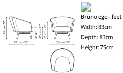
Bruno - feet Width: 83cm Depth: 83cm Height: 75cm
