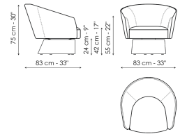
Bruno - covered base Width: 83cm Depth: 83cm Height: 75cm
